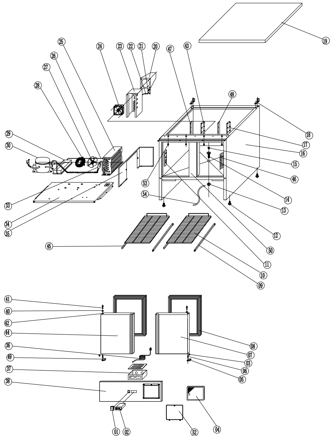
EXPLODE OF E-G-S901
