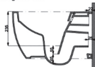
SECTION_VIEW A-A
